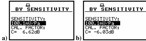
Displays during setting the sensitivity higher than 50.0 mV / Pa (a) and after pressing <ENTER> push-button with the calibration factor calculated (b)
