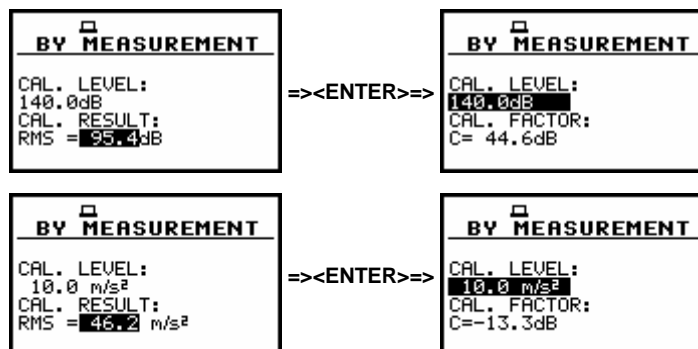
Displays after pressing <ENTER> push-button (after calculation of the calibration factor value)
